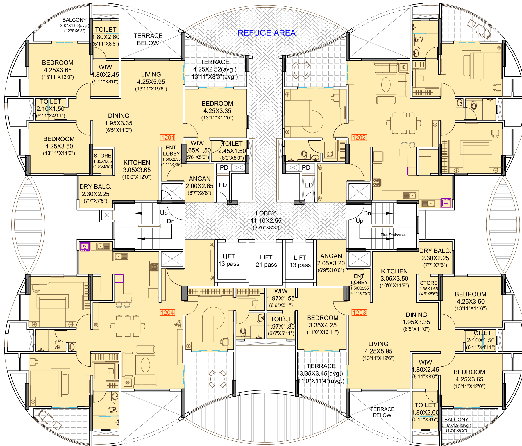
12TH FLOOR PLAN
