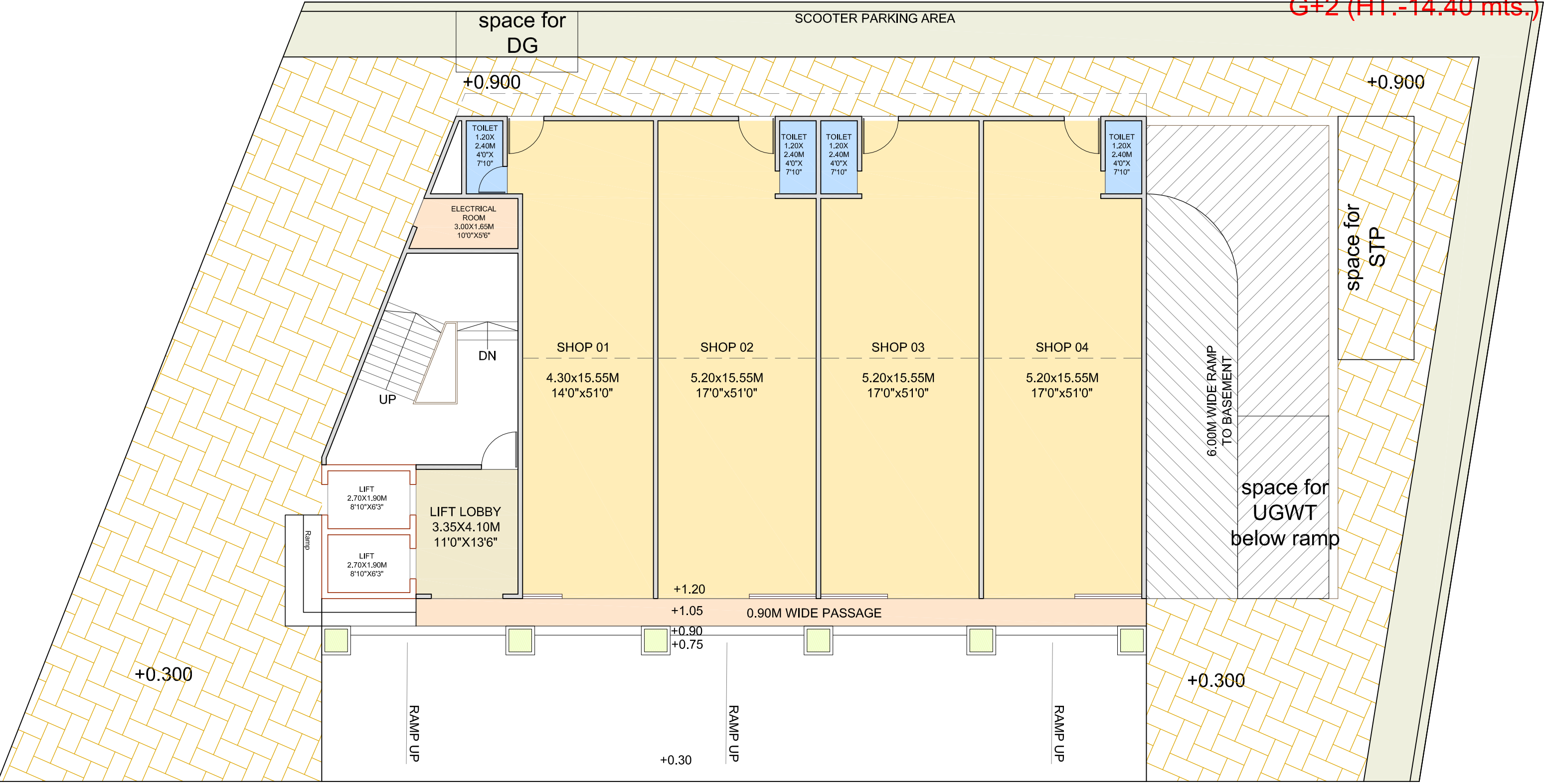
ROAD GROUND FLOOR PLAN
