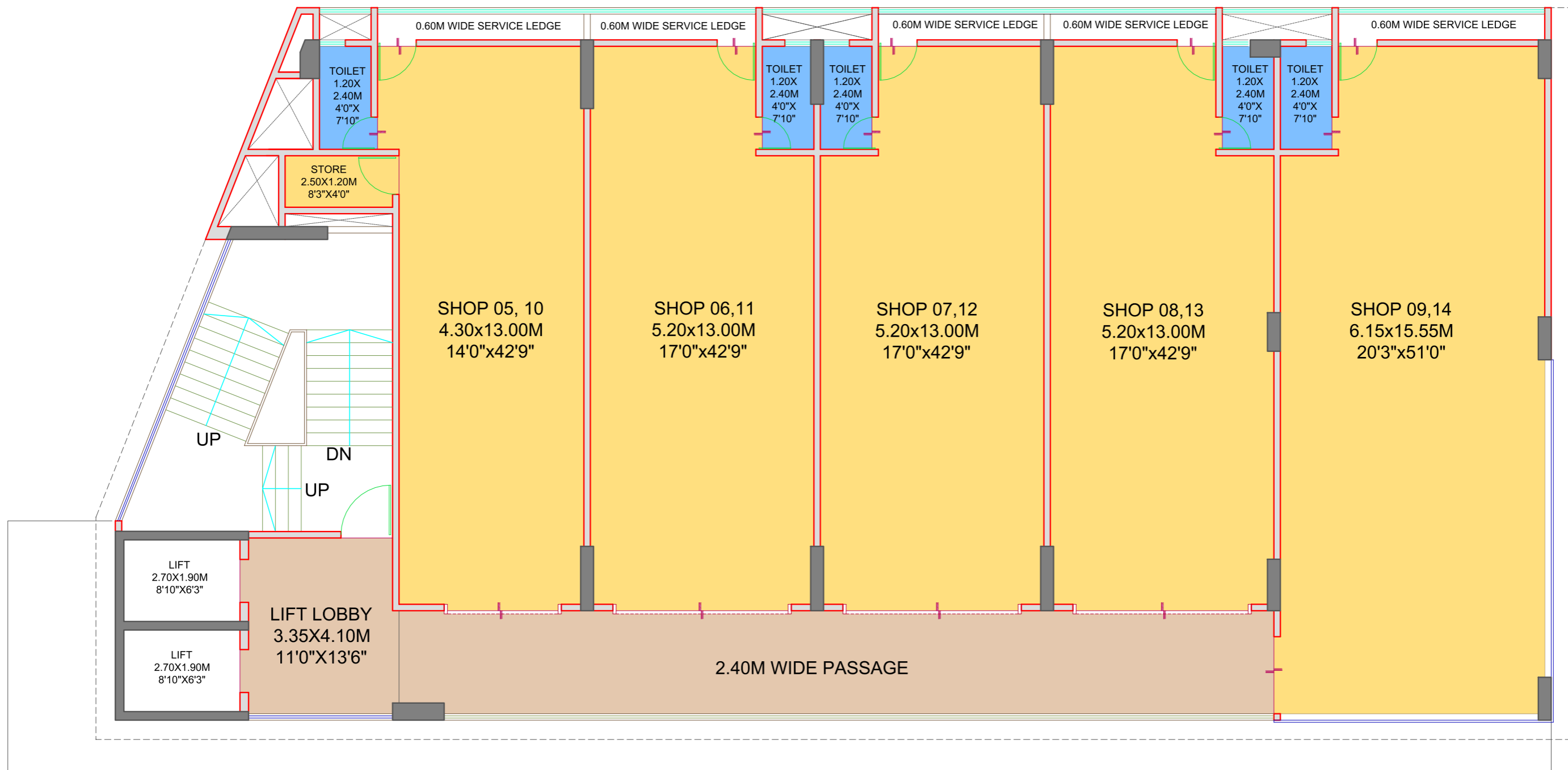
TYPICAL FIRST AND SECOND FLOOR PLAN
